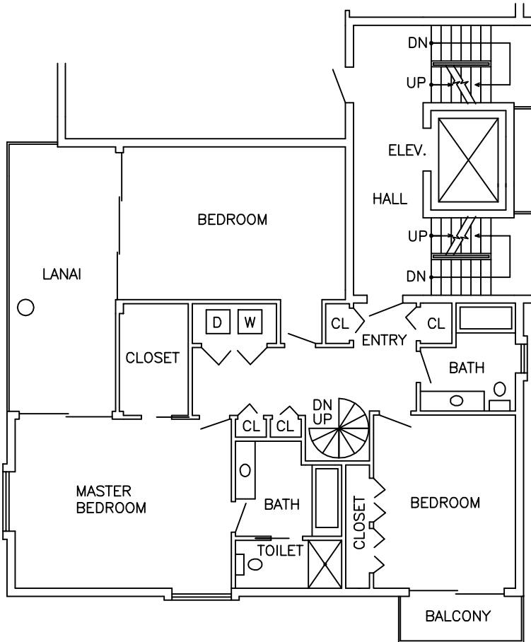
TRIPLEX UNIT 4A 2nd FLOOR PLAN 0' 3' 6' 12' Approximate Scale: 1" = 12'
